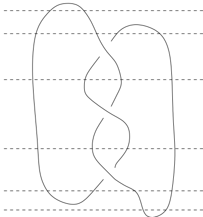
Fig. 1. knot diagram
