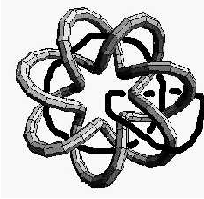
Fig. 4. link complement
