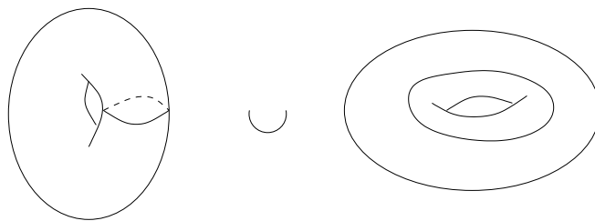
Fig. 2. Heegaard decomposition of the sphere
