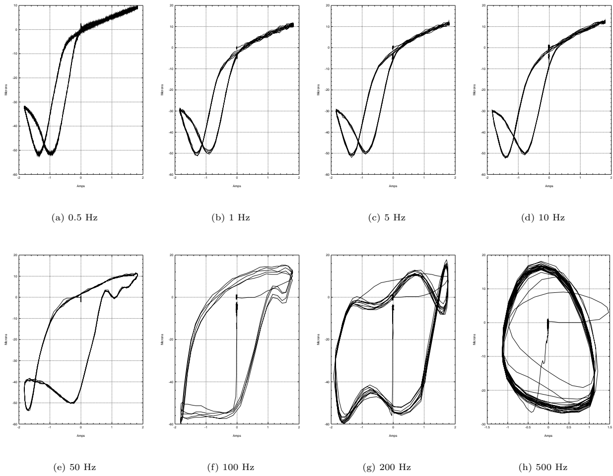
Figure 1: ETREMA MP 50/6 Actuator displacement (Microns) vs current (Amps) characteristic at different driving frequencies .
