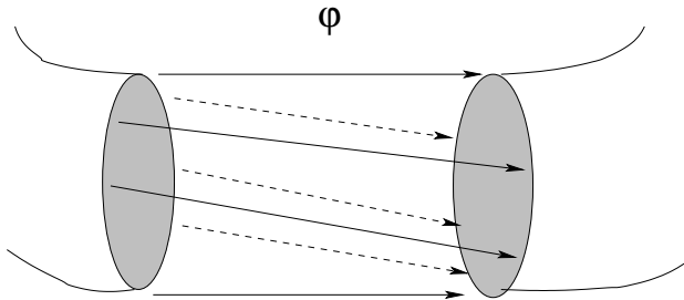
FIGURE 3. The welding map \varphi constructed in the proof of Theorem 3.1 glues two points of \gamma^+ back to their original positions and then “pulls” the remainder of \gamma^+ away from one fixed point and toward the other.
