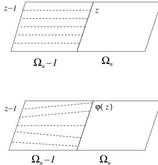
FIGURE 13. We extend \varphi_n to all of \Omega_{\tau_n} - 1 by acting on horizontal geodesics with endpoints on \gamma_n^+ .
